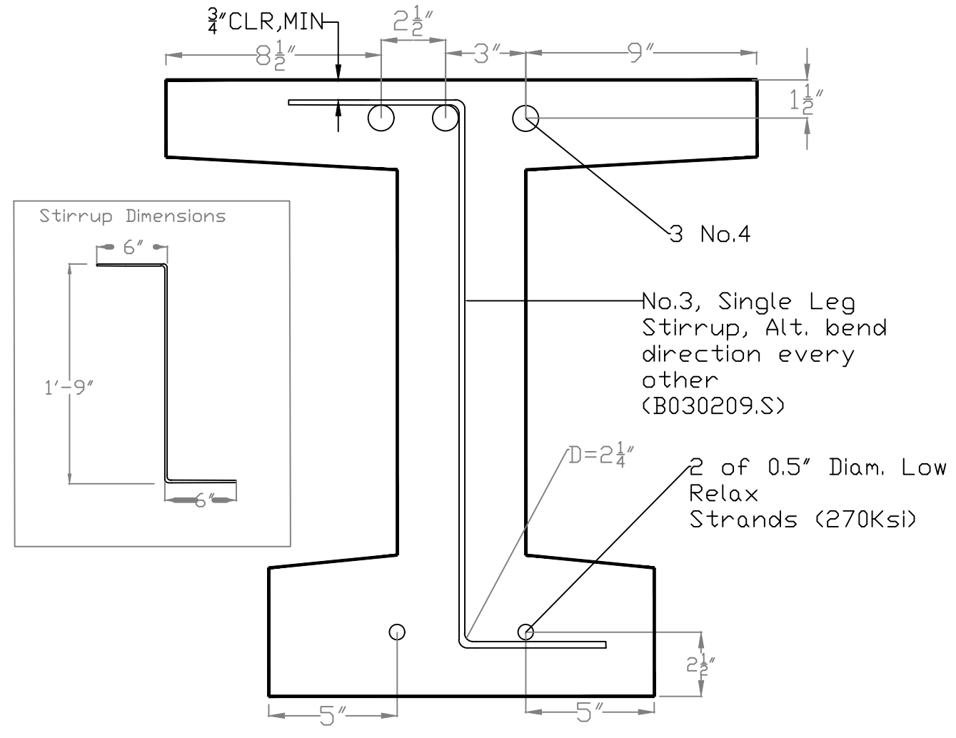
Section: Reinf. Details 3/4"=1'-0"
