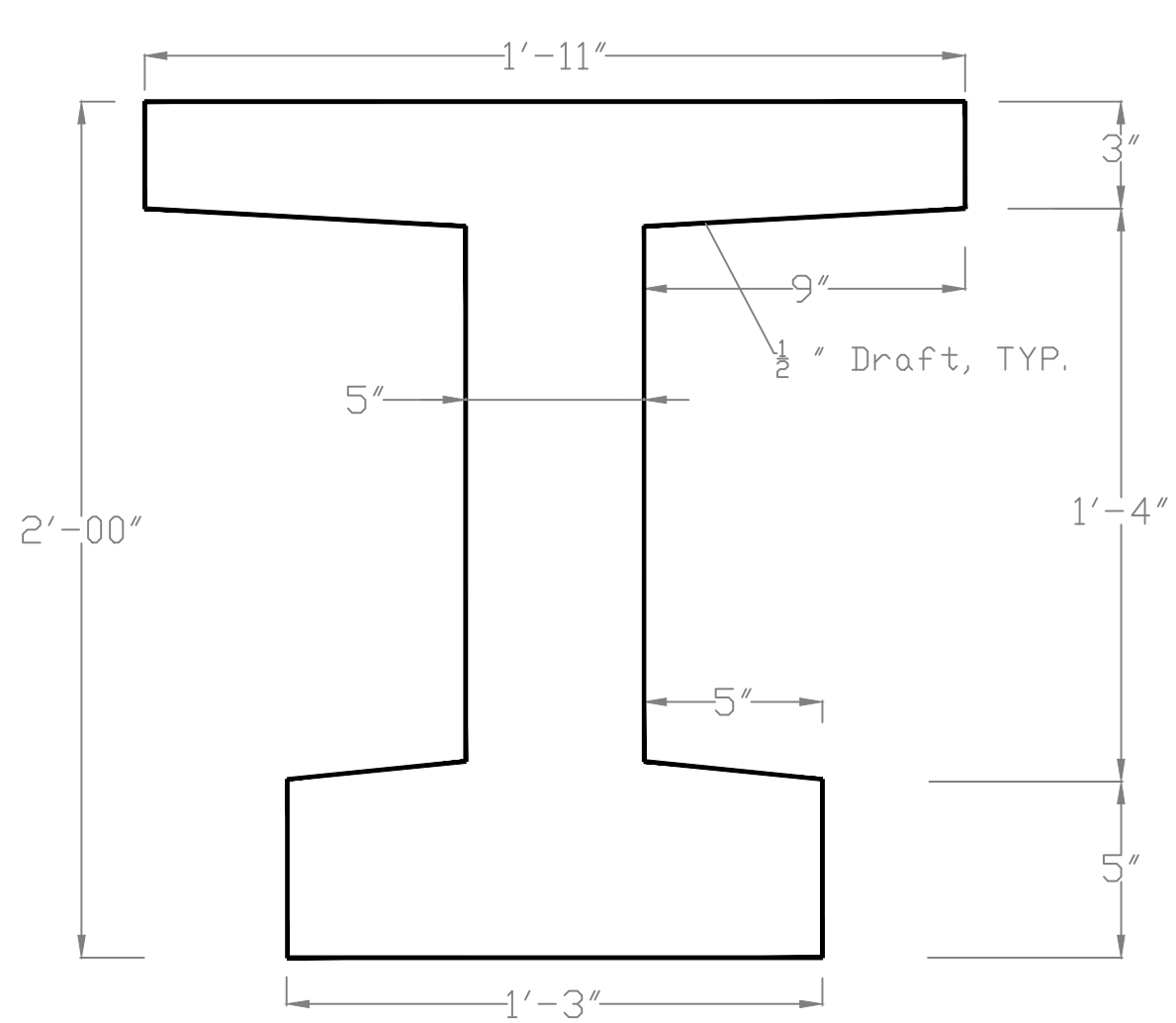
Section Dimensions 3/4"=1'-0"
